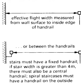
⑭ Minimum dimensions for stairs
